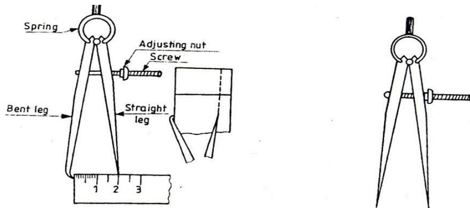
Figure 1.8: Odd leg caliper and divider
