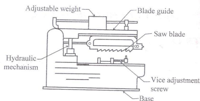
Figure 6.1 Power Hacksaw
