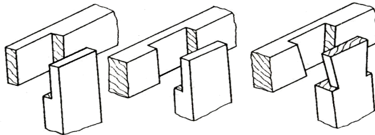
Figure 2.16: Lap joints
