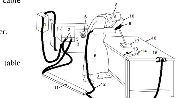
Fig1.The basic principle of arc welding
