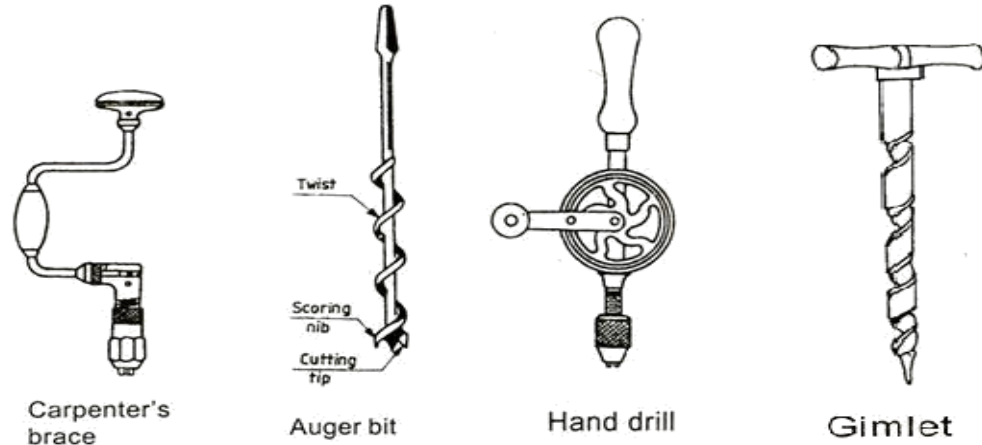
Figure 2.13: Drilling tools
