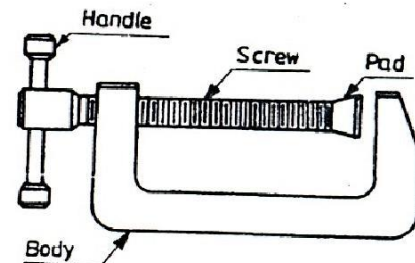
Figure 2.7: C-clamp
