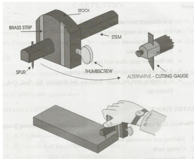
Marking gauge
