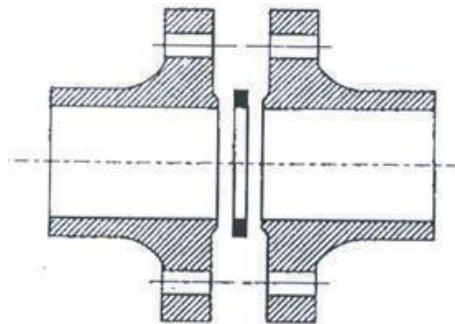
Flange joint.
