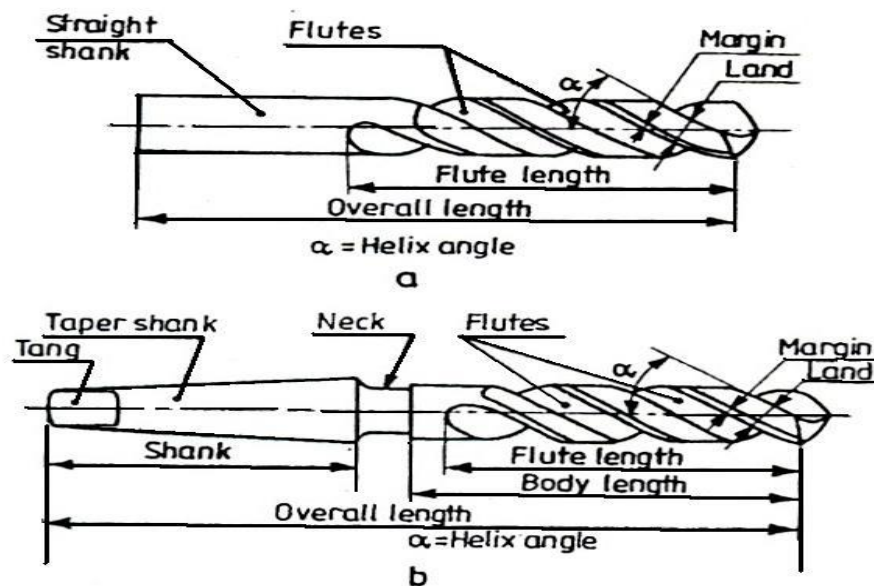
Figure 1.16: Twist drills
