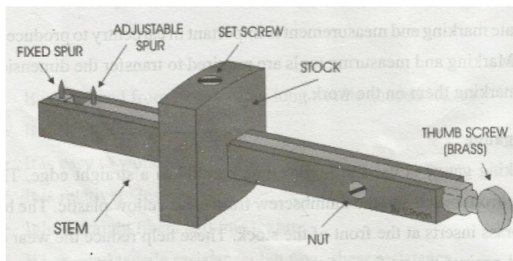
Mortise gauge
