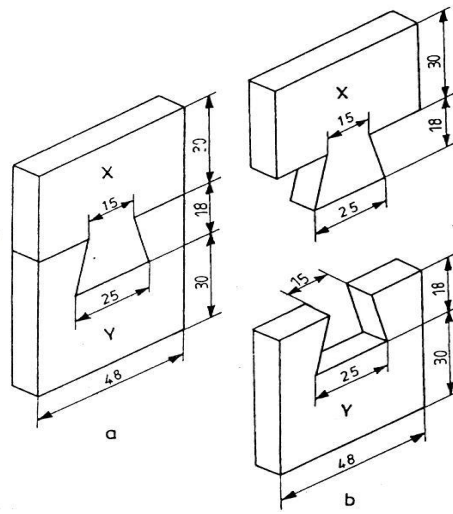
Figure 1.30: Dovetail Fitting
