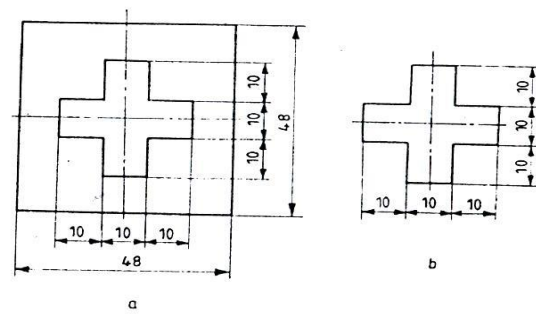
Figure 1.33: Cross fitting
