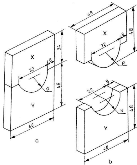
Figure 1.32: Half round fitting
