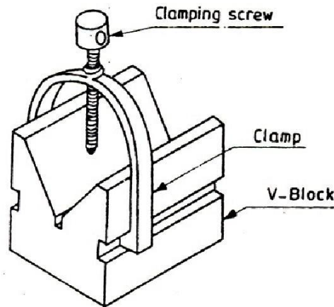
Figure 1.2: V-block
