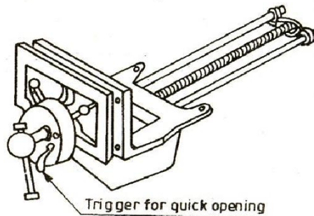
Figure 2.6: Carpenter's vice
