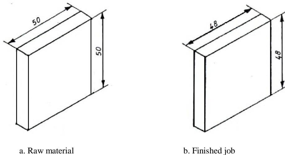
Figure 1.35: Square filing
