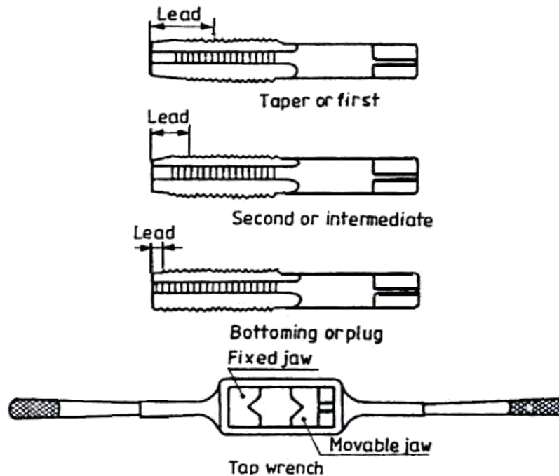
Figure 1.17: Taps and tap wrench
