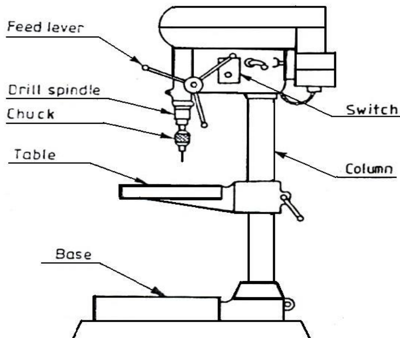
Figure 1.19: Bench drill
