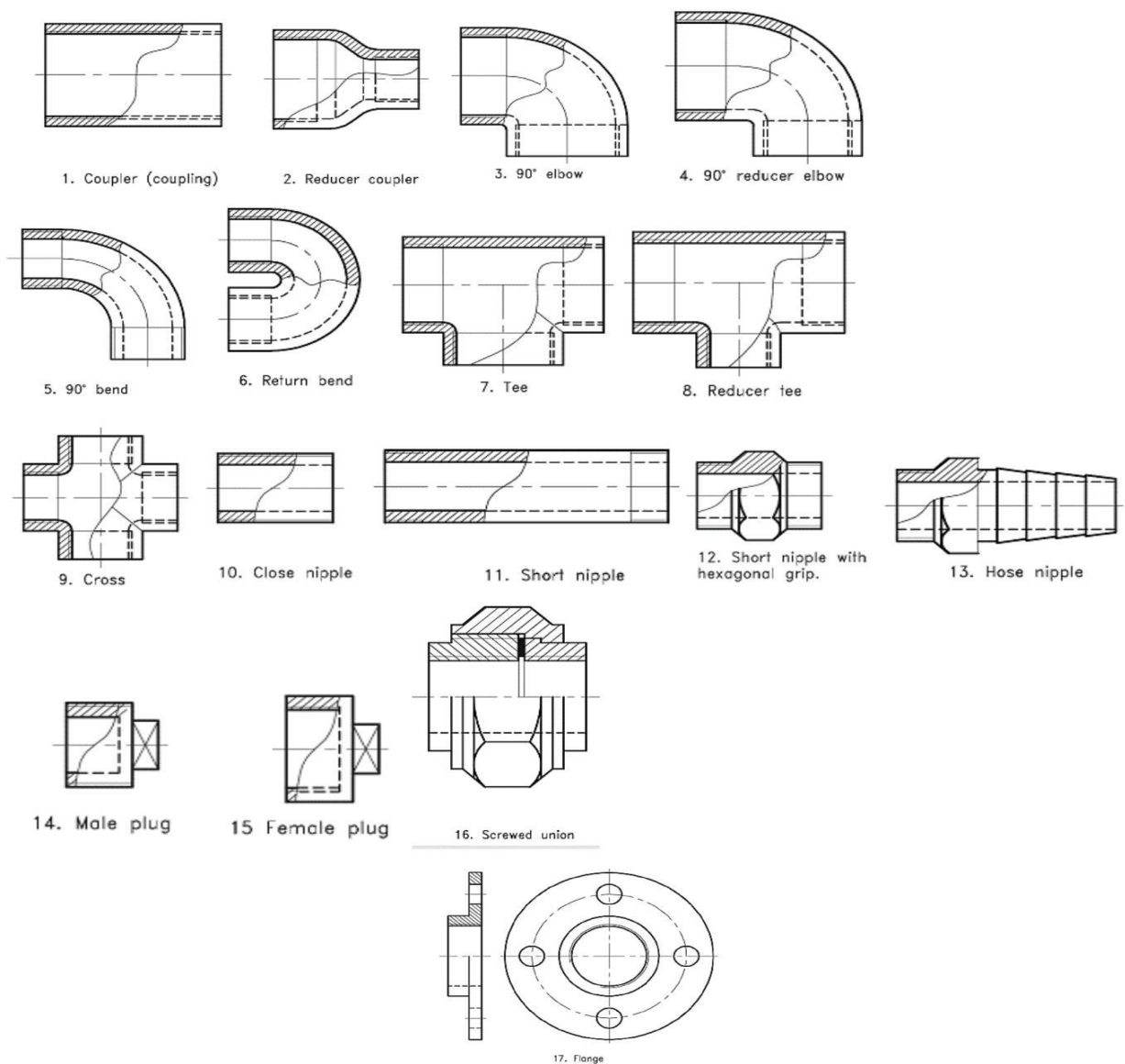
Figure 5.1: Various pipe joints.
