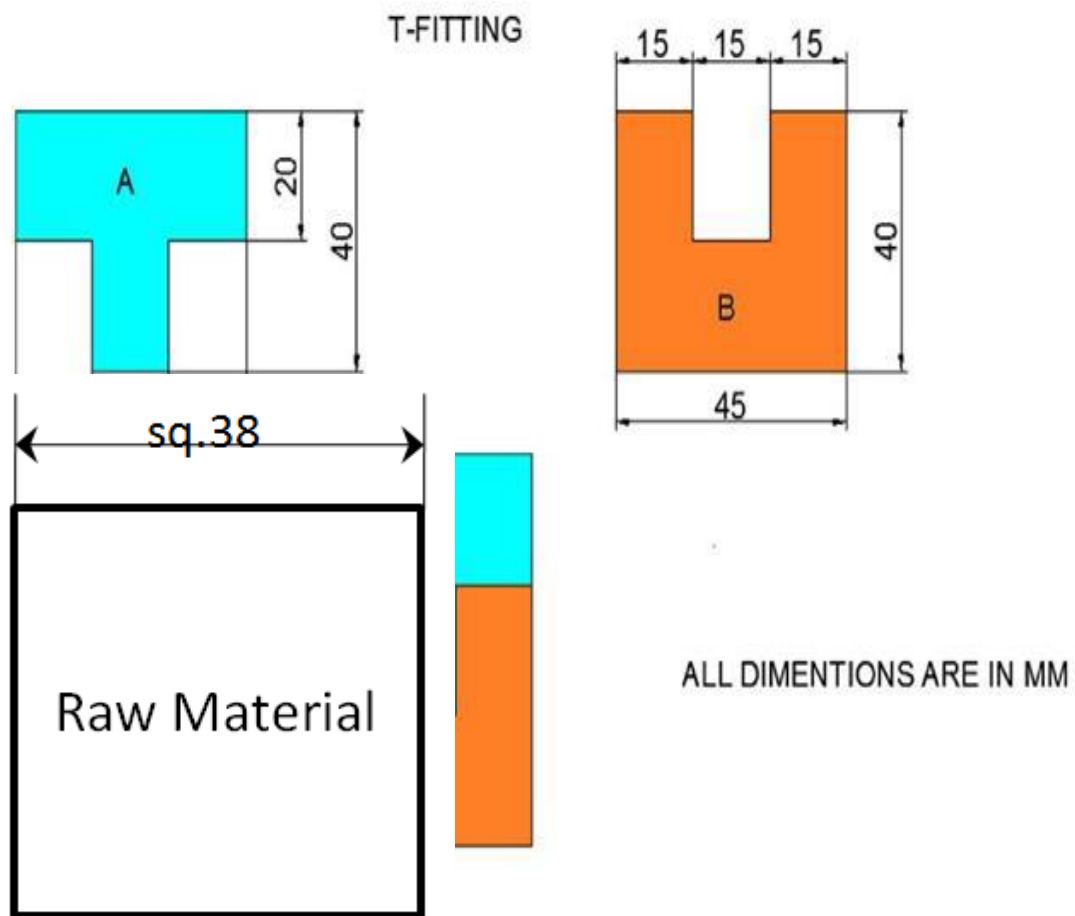
Figure 1.37: T-Fitting
