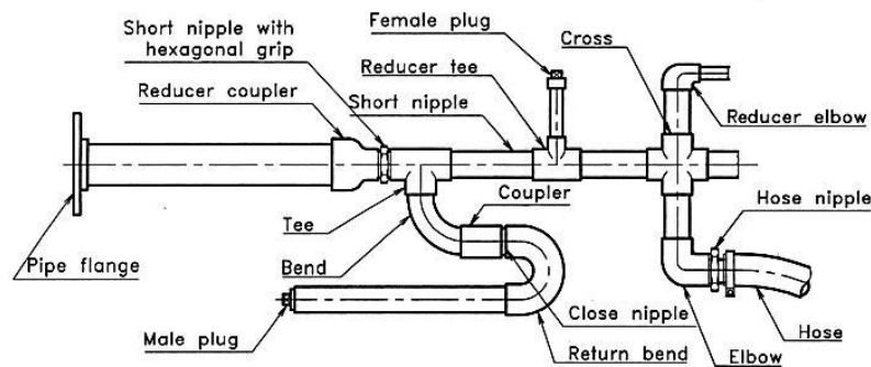
Figure 5.2: Application of various joints in the pipe fittings
