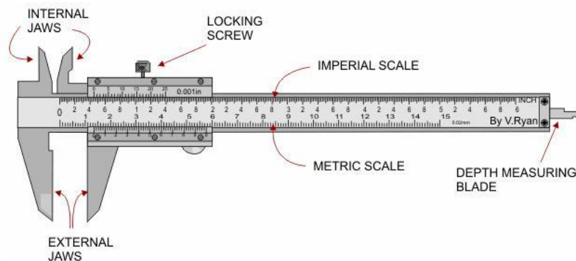
Figure 1.11: Vernier caliper
